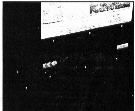
Galvanized Steel Hinge Roll and Stainless Steel Springs - Add strength and durability to the rack.
